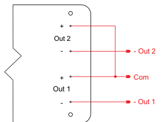
Outputs > 500Vdc
